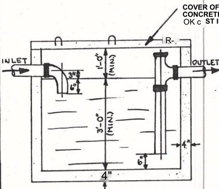
SECTION A-A CONCRETE BOX
