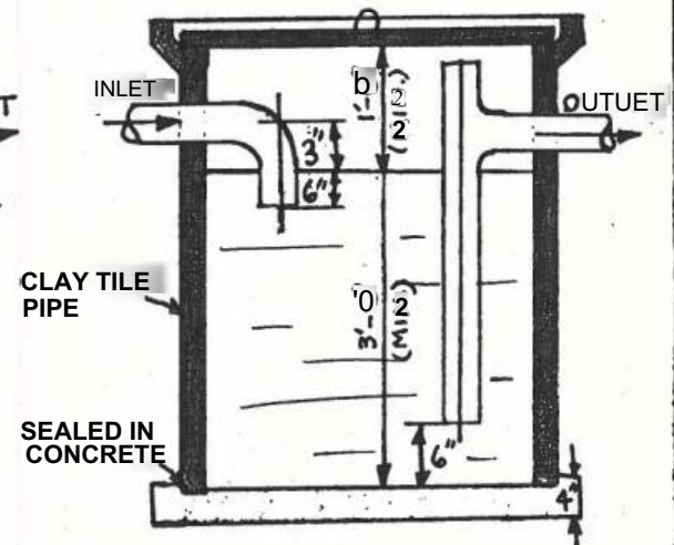
SECTION B-B CLAY TILE PIPE
